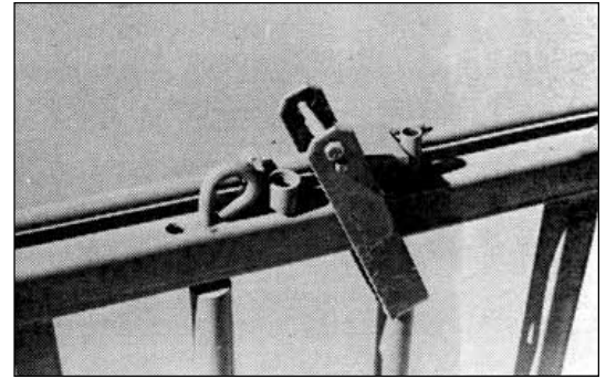
Pipe Stub can be placed over welded pin for locking in individual animals - simple & unique
